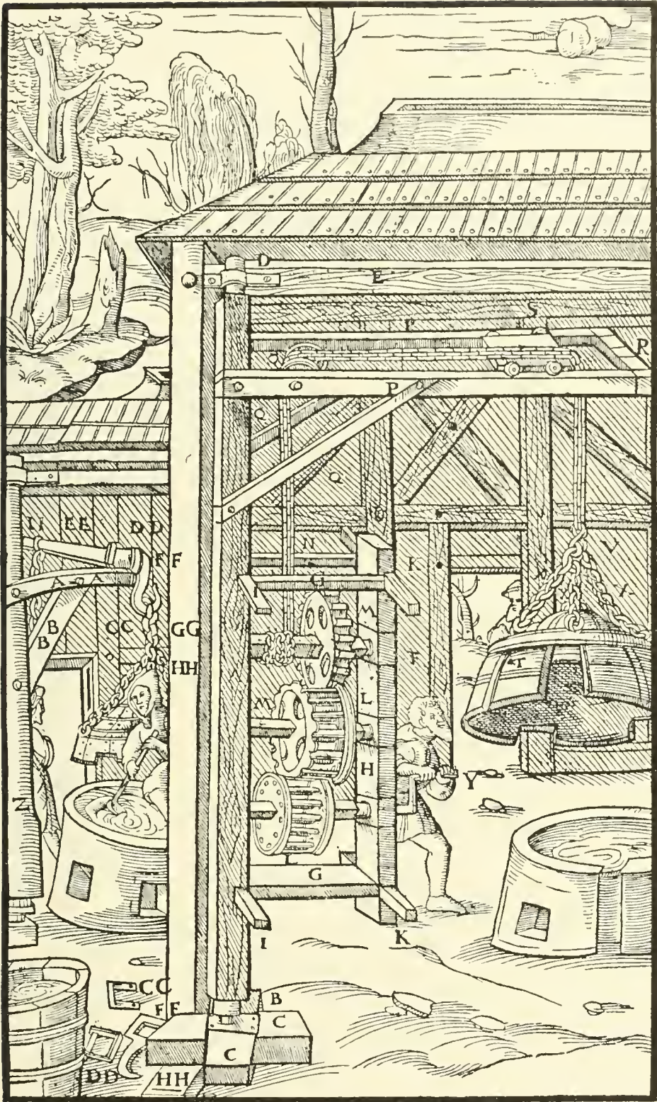
A—CRANE-POST. B—SOCKET. C—OAK CROSS-SILLS. D—BAND. E—ROOF-BEAM. F—FRAME. G—LOWER SMALL CROSS-BEAM. H—UPRIGHT TIMBER. I—BARS WHICH COME FROM THE SIDES OF THE CRANE-POST. K—BARS WHICH COME FROM THE SIDES OF THE UPRIGHT TIMBER. L—RUNDLE DRUMS. M—TOOTHED WHEELS. N—CHAIN. O—PULLEY. P—BEAMS OF THE CRANE-ARM. Q—OBLIQUE BEAMS SUPPORTING THE BEAMS OF THE CRANE-ARM. R—RECTANGULAR IRON PLATES. S—TROLLEY. T—DOME OF THE FURNACE. V—RING. X—THREE CHAINS. Y—CRANK. Z—THE CRANE-POST OF THE OTHER CONTRIVANCE. AA—CRANE-ARM. BB—OBLIQUE BEAM. CC—RING OF THE CRANE-ARM. DD—THE SECOND RING. EE—LEVER-BAR. FF—THIRD RING. GG—HOOK. HH—CHAIN OF THE DOME. II—CHAIN OF THE LEVER-BAR
